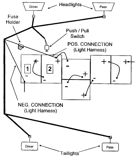
Yamaha Basic 36-Volt Wiring Diagram
